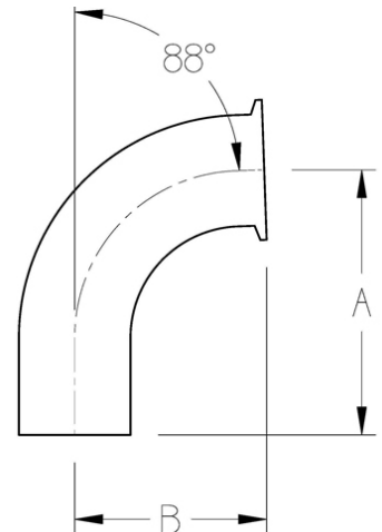
TA88CMS – Automatic Tube Weld x Short Hygienic Clamp Joint 88 Deg Elbow
