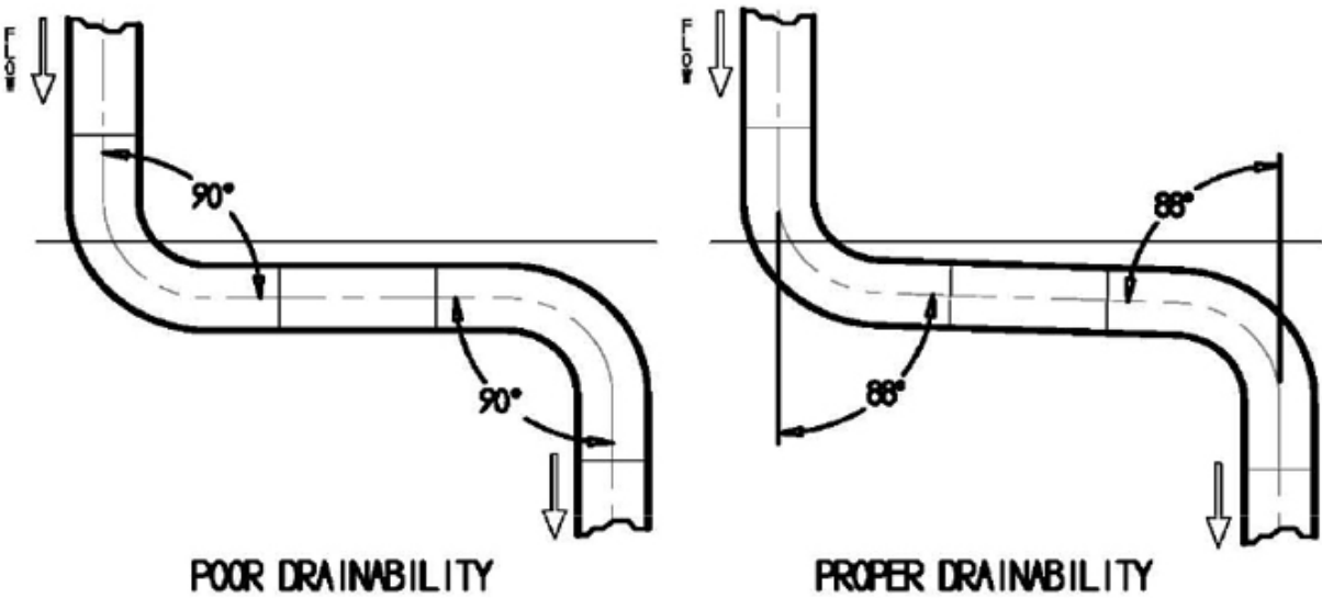
88 and 92 degree Elbows
